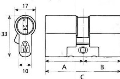
Double Key & Thumbturn Cylinder
