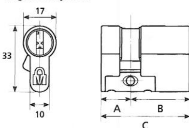
Single Half Cylinder
